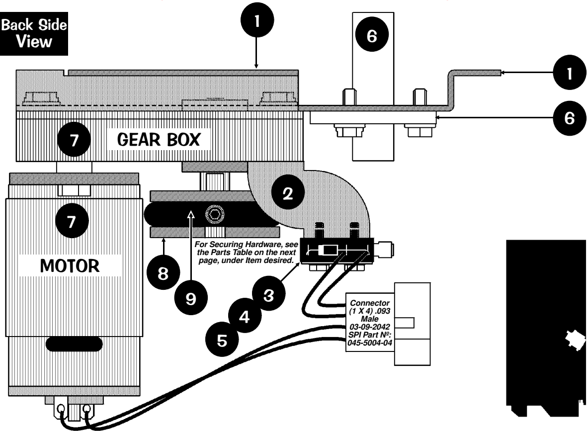
Bottom View
